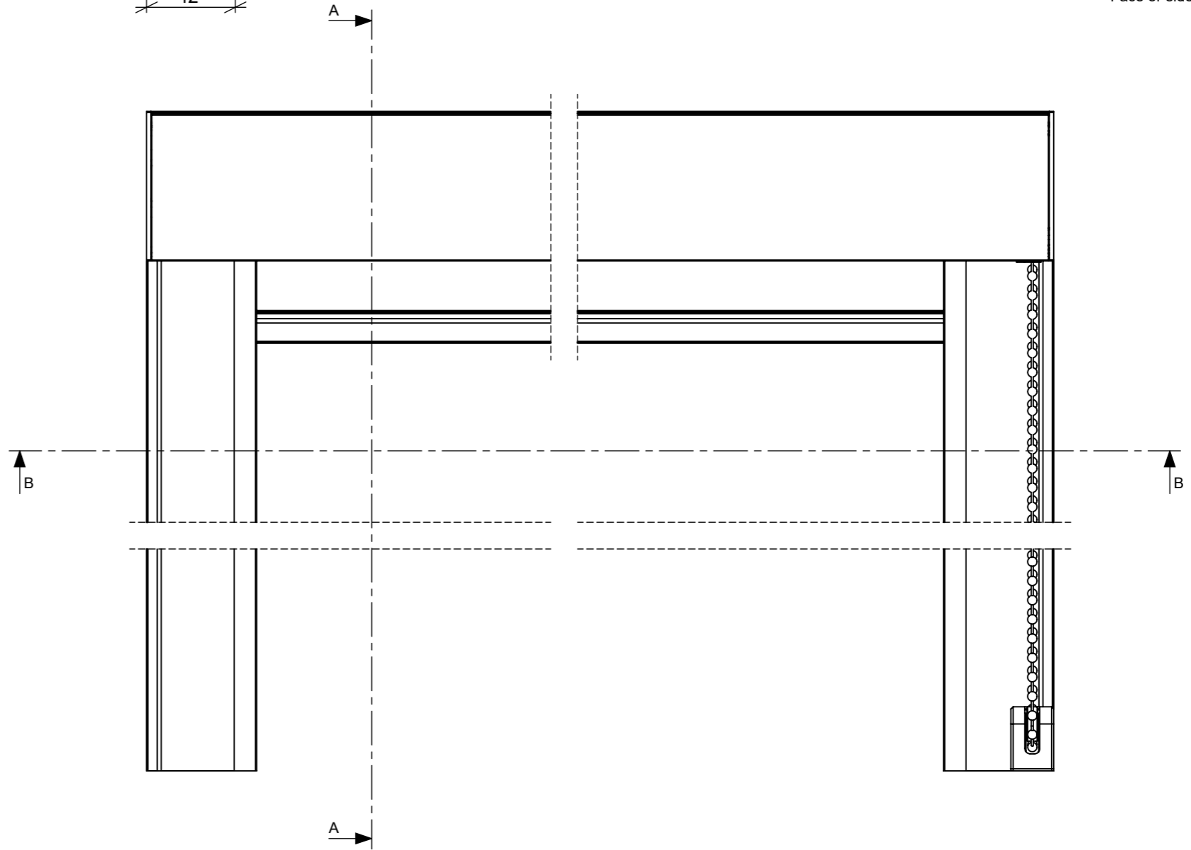
Side or Face Mount - Single Seal SECTION B-B
