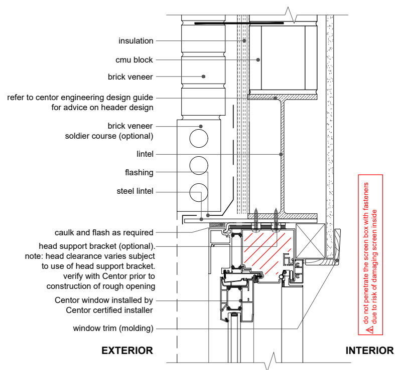
2 head detail section
