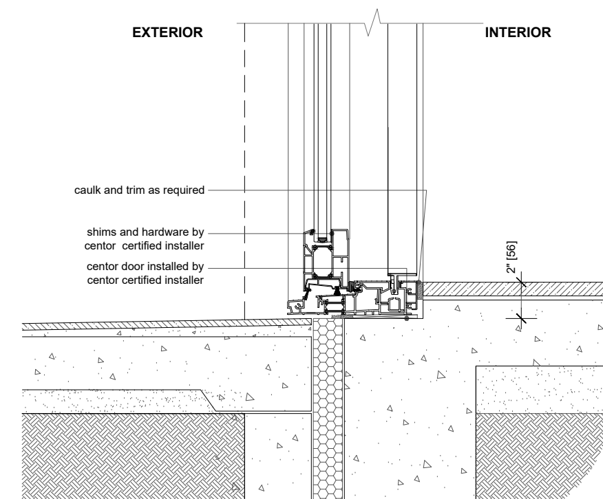
typical rough opening clearances
